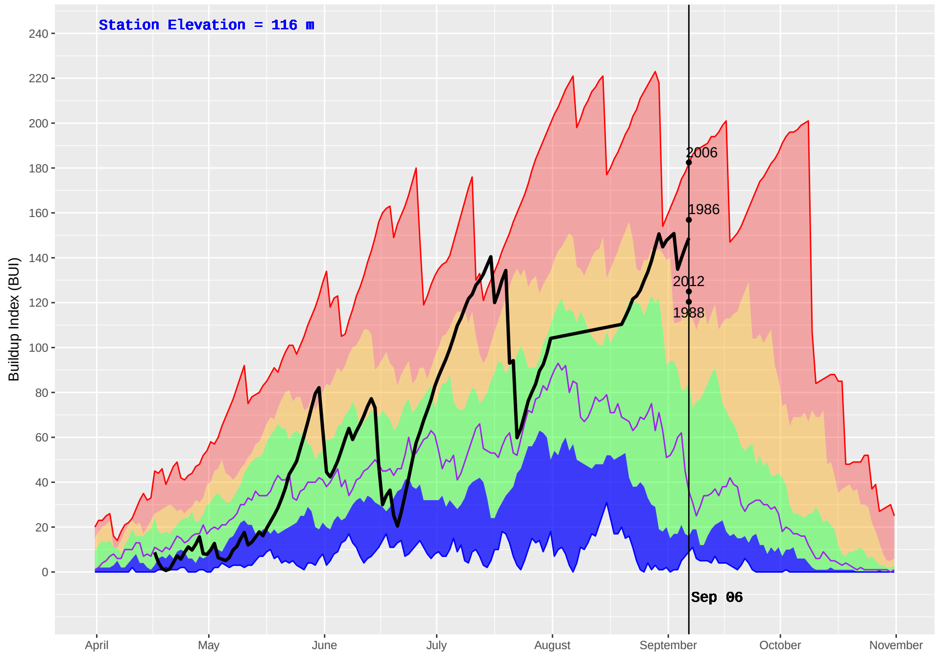
SCAR CREEK (82) : Historical (1982–2016) and Current (2017) Noon Buildup Index (BUI)
