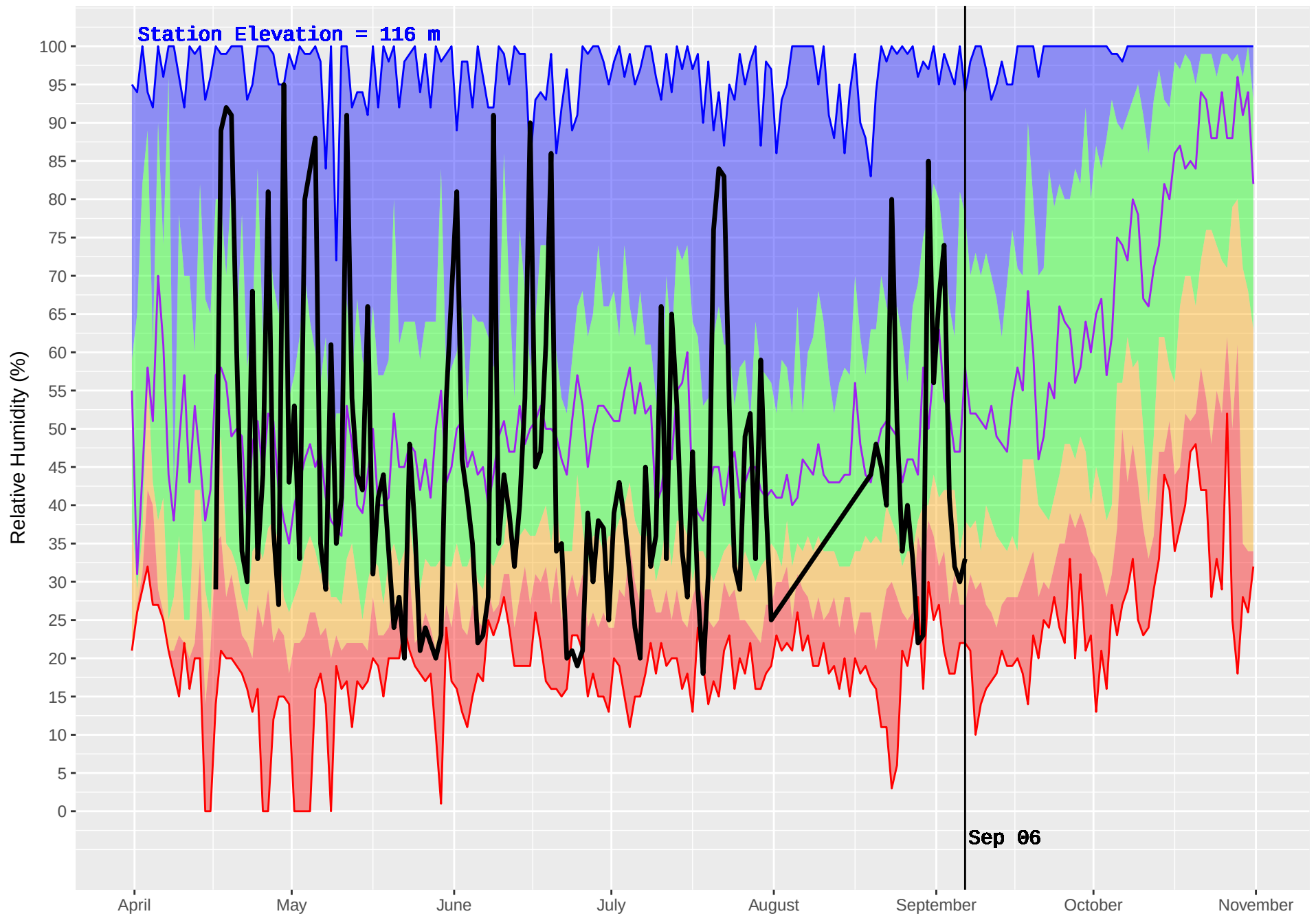
SCAR CREEK (82) : Historical (1982–2016) and Current (2017) Noon Relative Humidity
