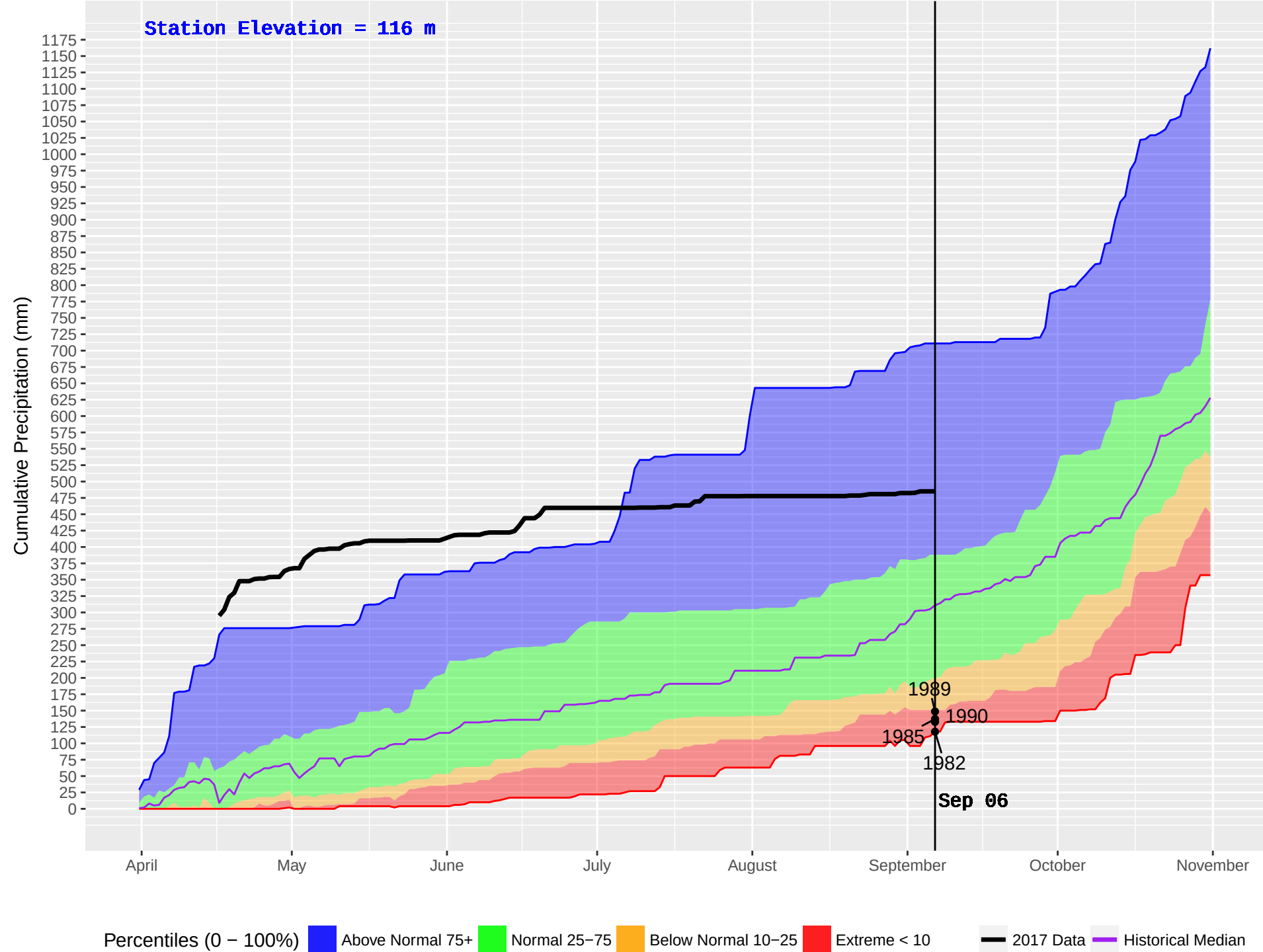
SCAR CREEK (82) : Historical (1982–2016) and Current (2017) Noon Cumulative Precipitation
